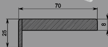
ADJUSTABLE ARCHITRAVE (MDF) 70(17)x8x2150mm
