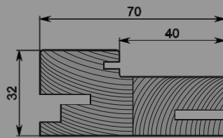
ADJUSTABLE DOOR FRAME (wood) 70x32x2070mm
