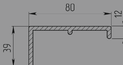
ADJUSTABLE ARCHITRAVE (composite) 80x12x2150mm
