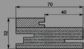
ADJUSTABLE DOOR FRAME (plywood + MDF) 70x32x2070mm
