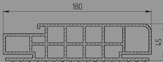
ADJUSTABLE DOOR FRAME (composite) 180x45x2070mm
