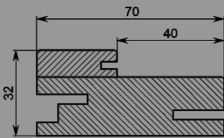
ADJUSTABLE DOOR FRAME (MDF) 70x32x2070mm
