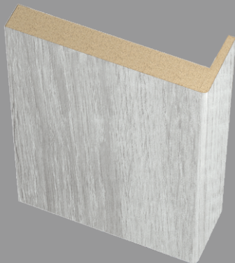
ADJUSTABLE DOOR FRAME (MDF) 70x32x2070mm
